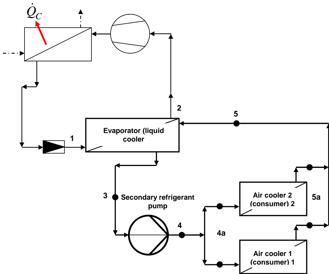
Fig. 6: Indirect cooling system, simplified diagram
