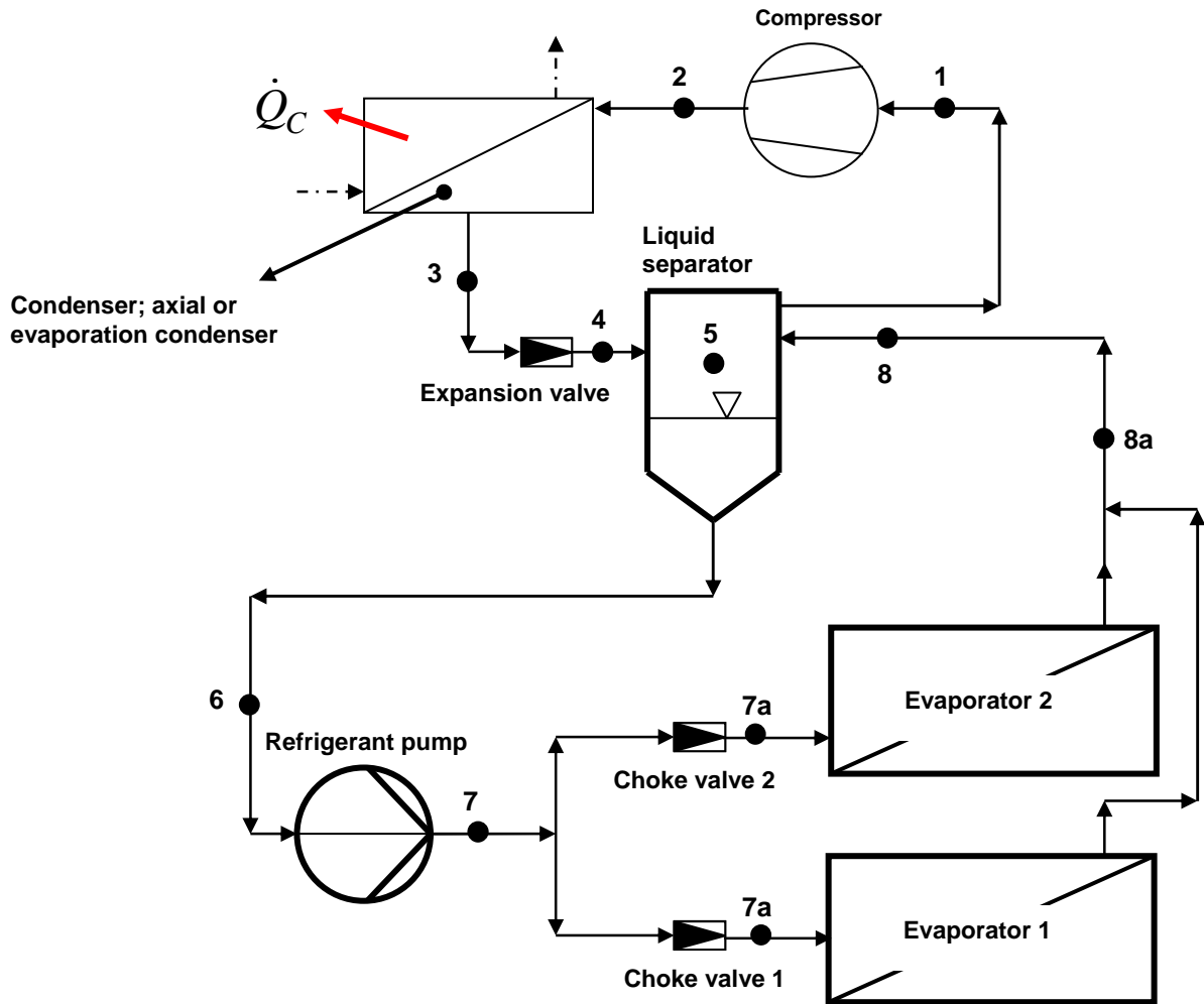
Fig. 5: Pump circuit, simplified diagram
