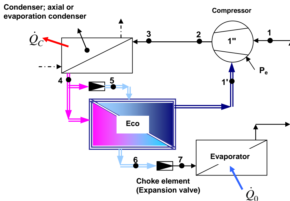
Fig. 4: Single-stage refrigerant circuit with economizer operation; simplified diagram
