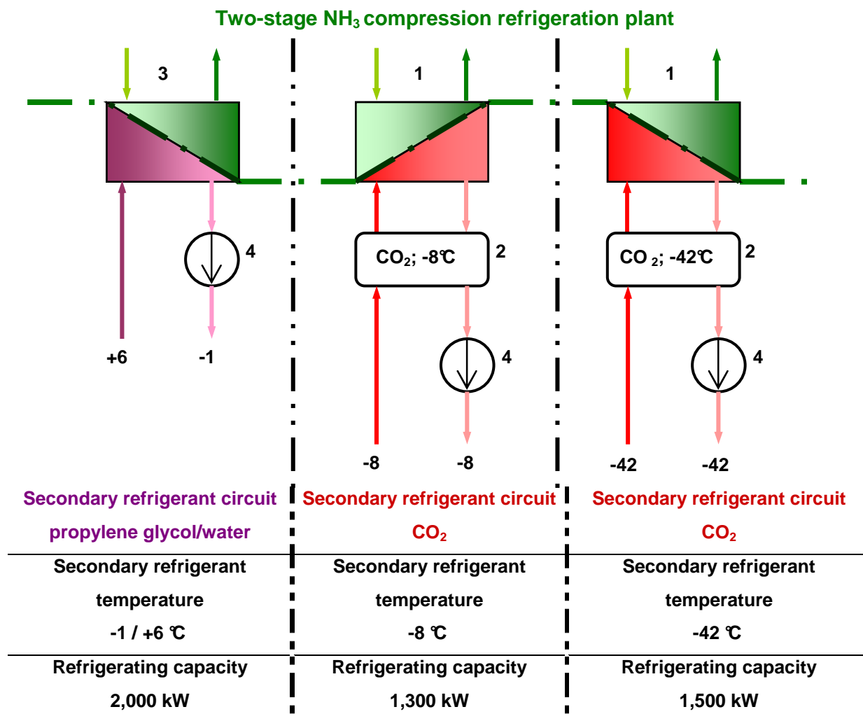
Fig. 8: Simplified diagram of the secondary refrigerant circuit for fish processing in Sassnitz, Germany
