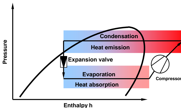
Fig. 2: Cyclic process of a refrigeration plant in the lg p, h-diagram
