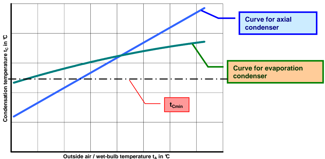
Fig. 7: Condensation temperature t_c (range +20 to +50 °C) over outside air temperature t_A (-15 to +35 °C) and wet bulb temperature t_F (0 to +23 °C)
